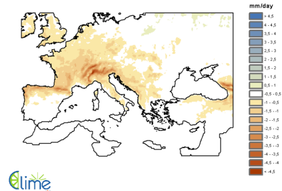
Figure 3: Illustrative downscaled projection for Precipitation in JJA under RCP8.5. The map shows projected rainfall for 2071-2100 (expressed relative to the 1971-2000 base period).
