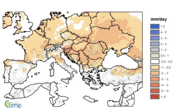
Figure 4: Illustrative validation of downscaled precipitation climatology in JJA (model minus observed), for 1971-2005. Model is at 14km spatial resolution
