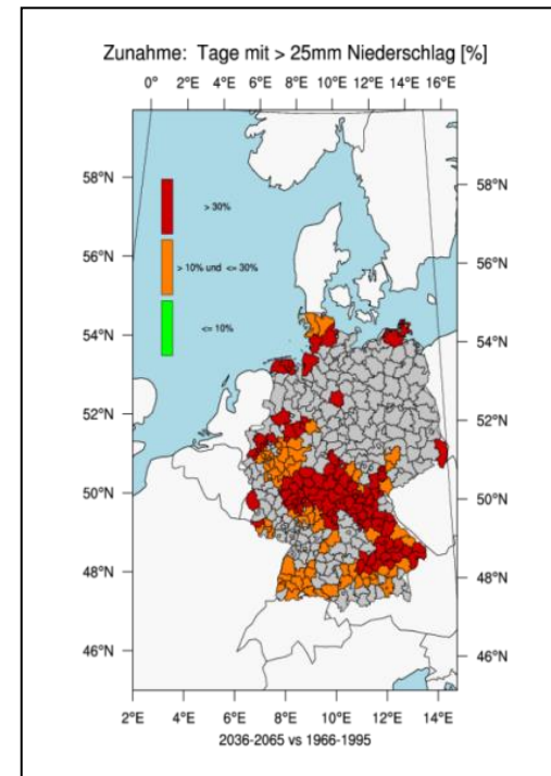
Figure 2 Example of Prototype product: 2036-2065, days with more than 25mm precipitation: All regions that failed at least one robustness test are coloured in grey.
